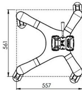
4 Wheel base
