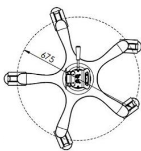
5 Wheel base
