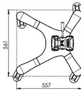
4 Wheel base
