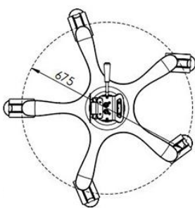
5 Wheel base
